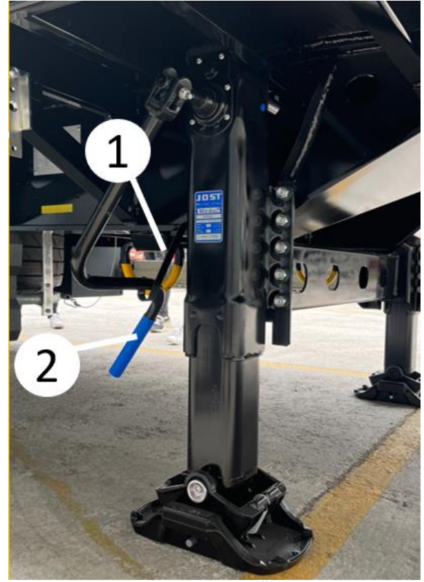
Mekanik ayak
